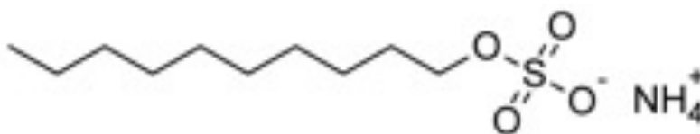
Molecular Structure
